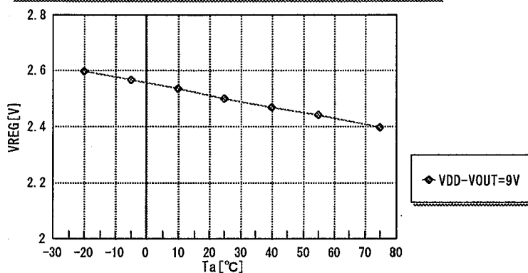
VREG vs. Temperature (Typical performance)
