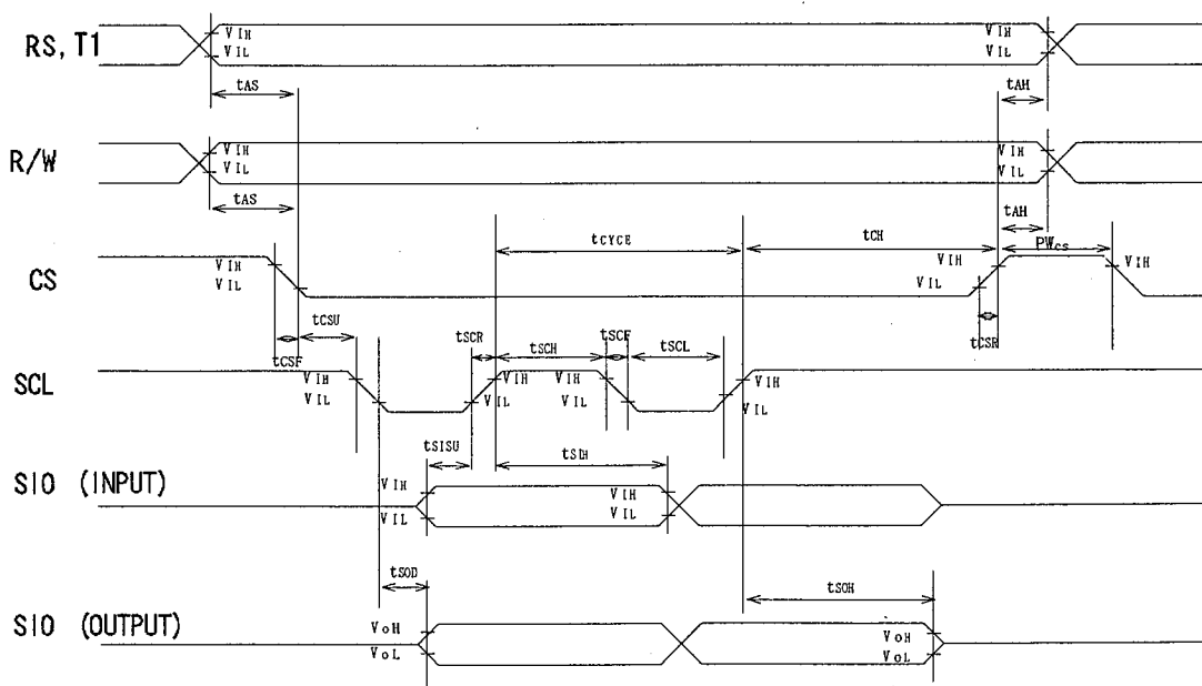
The timing characteristics of the serial bus write/read operating sequence
