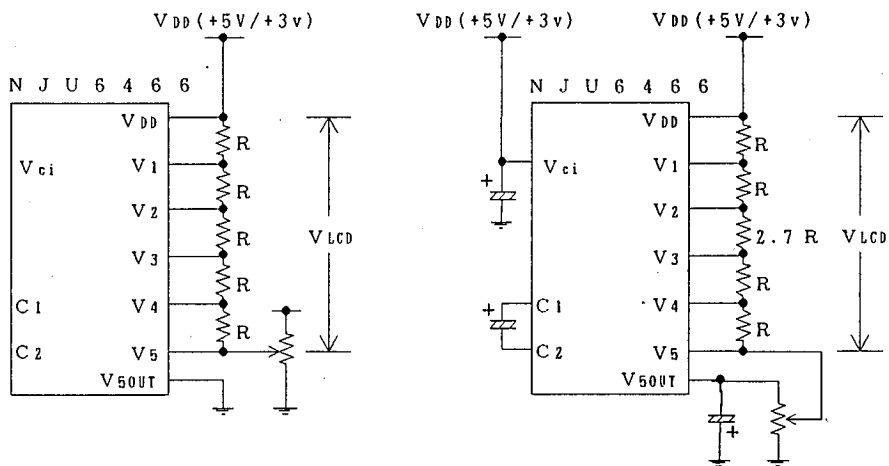
(a) 1/5 bias (1/16 Duty) (Internal Voltage Doubler No-use example) (b) 1/6.7 bias (1/32 Duty) (Internal Voltage Doubler using example)
