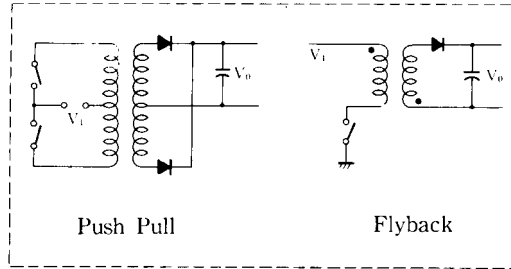
Transformer-Coupled Outputs
