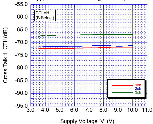
Input Cross Talk 1 vs. Supply Voltage
