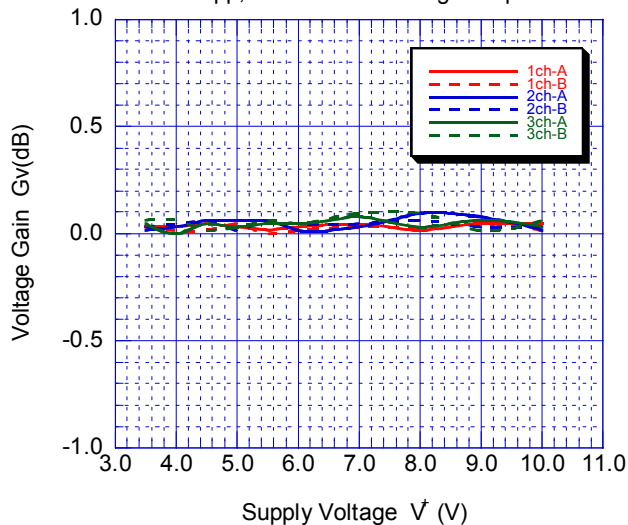
Channel Gain Defference vs. Supply Voltage
