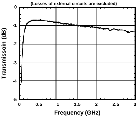
ANT Port to GSM900 Rx Port Transmission Characteristics (VDD=2.7V, VCTL=0/2.7V) (Losses of external circuits are excluded)
