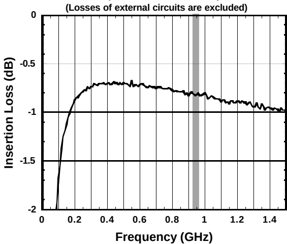
ANT Port to GSM900 Rx Port Insertion Loss vs. Frequency (VDD=2.7V, VCTL=0/2.7V) (Losses of external circuits are excluded)
