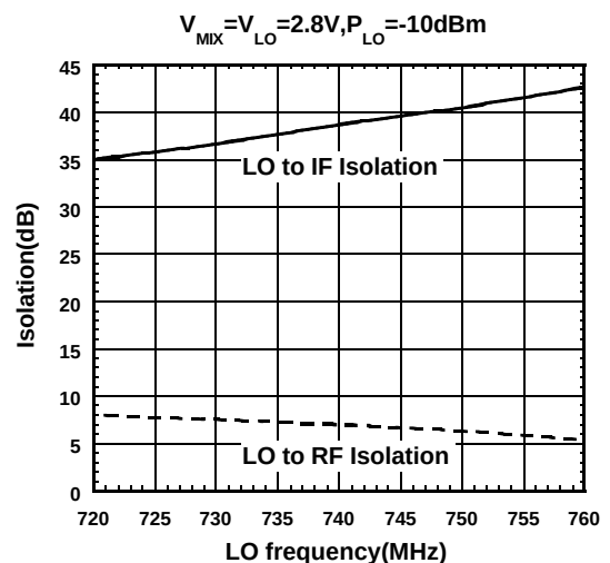
Isolation vs. LO frequency
