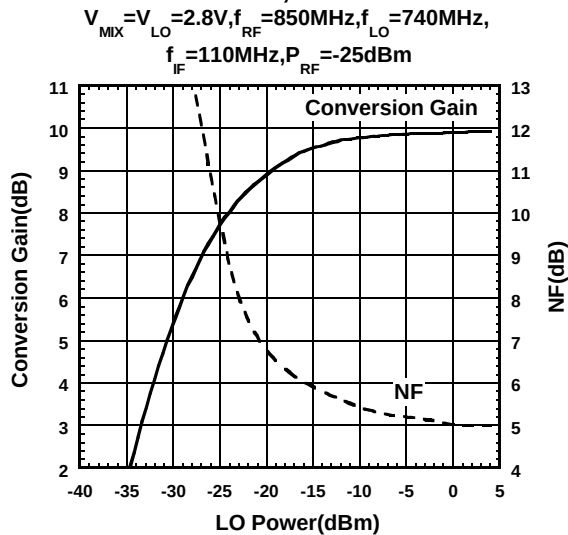
Conversion Gain, NF vs. LO Power
