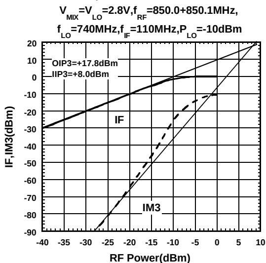
IF, IM3 vs. RF Power
