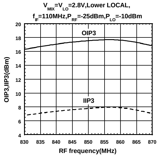
OIP3, IIP3 vs. RF frequency
