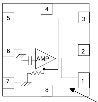
HB3 Type (Top View)
