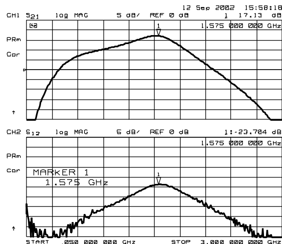
S 21 , S 12
