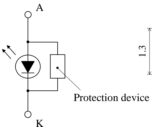
Internal Circuit
