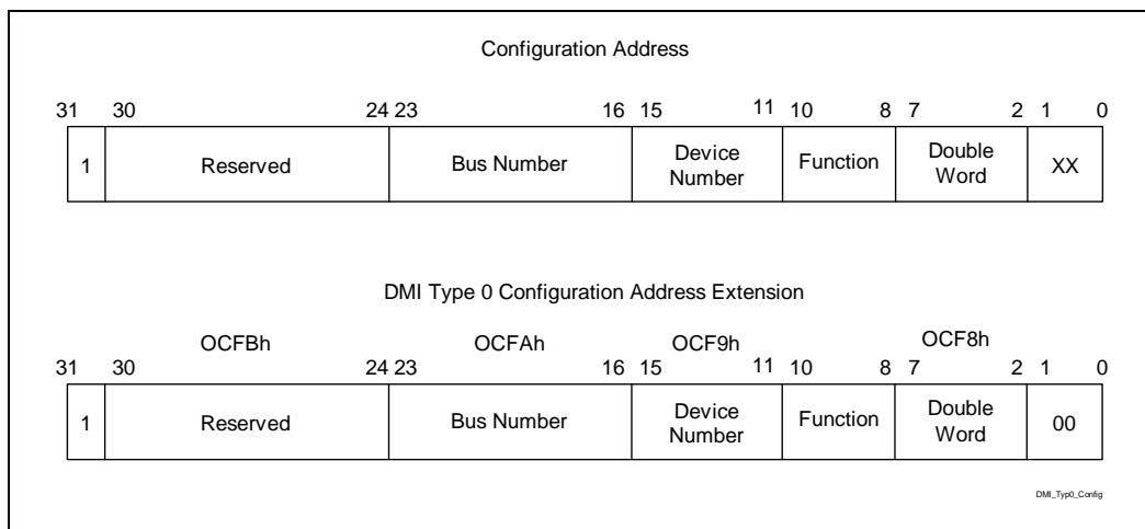
Figure 3-2. DMI Type 0 Configuration Address Translation
