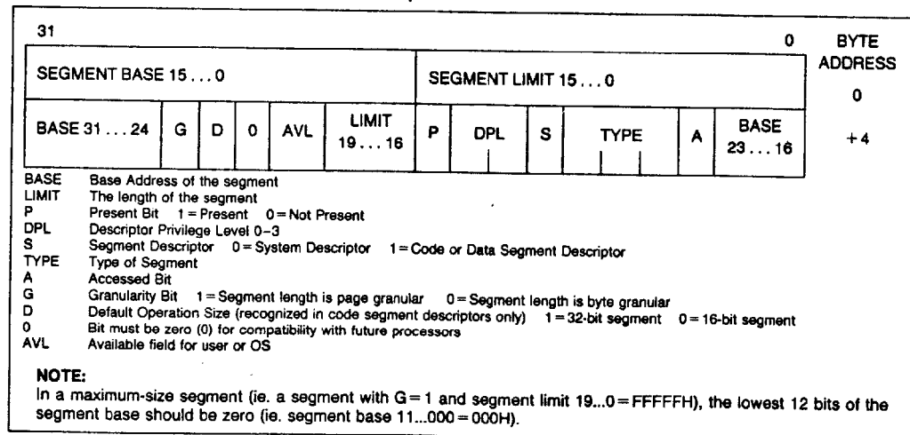
Figure 4-5. Segment Descriptors
