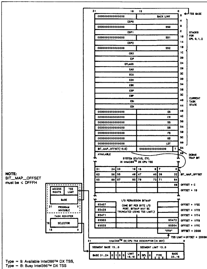
Figure 4-15a. Intel386™ DX TSS and TSS Registers
