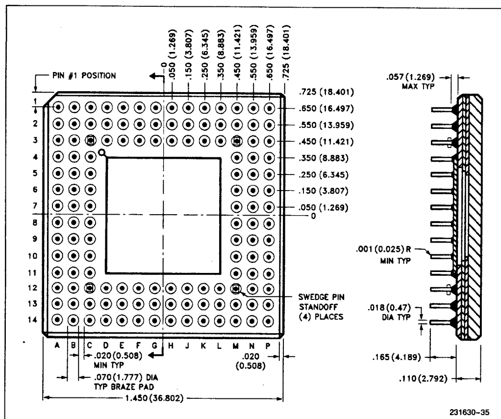
Figure 8.1. 132-Pin Ceramic PGA Package Dimensions
