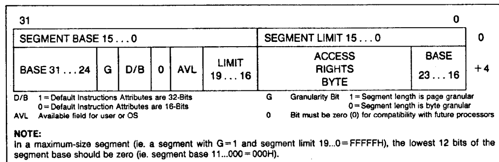
Figure 4-6. Segment Descriptors
