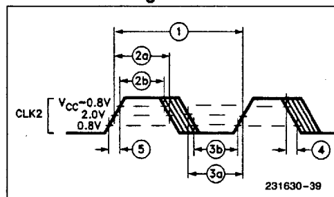
Figure 9-3. CLK2 Timing
