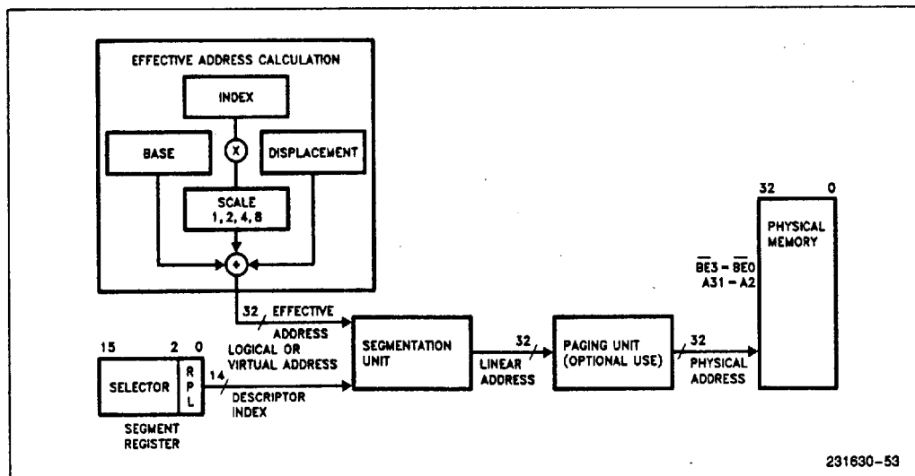
Figure 2-11. Address Translation
