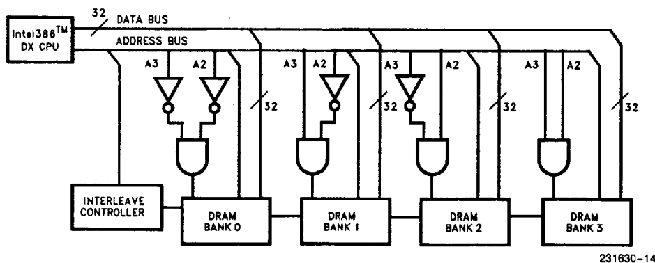
Figure 5-10. 2-Bank and 4-Bank Interleaved Memory Structure
