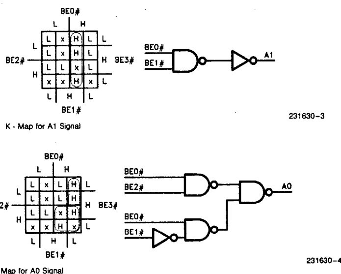
Figure 5-3. Logic to Generate A0, A1 from BE0 #-BE3 #
