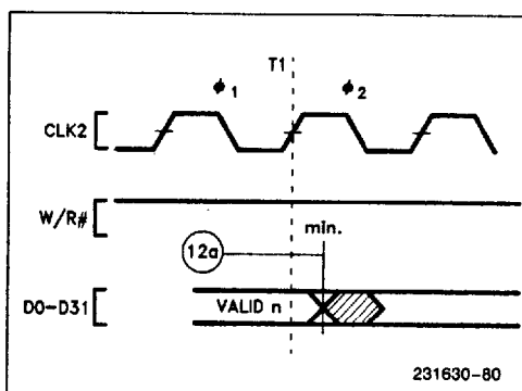
Figure 9-5b. Write Data Hold Timing (25 MHz, 33 MHz)
