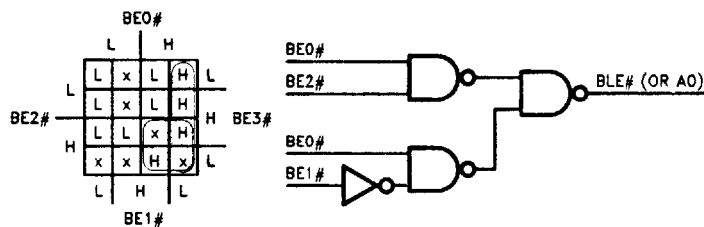
Figure 5-7. Logic to Generate A1, BHE# and BLE# for 16-Bit Buses
