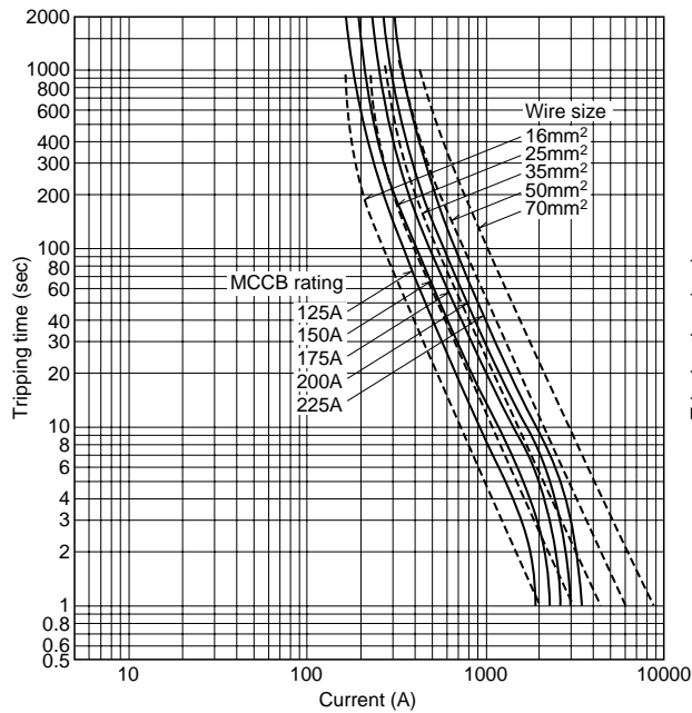
c) 225A-fream MCCB
