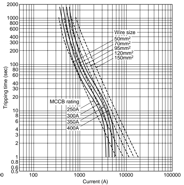
d) 400A-fream MCCB
