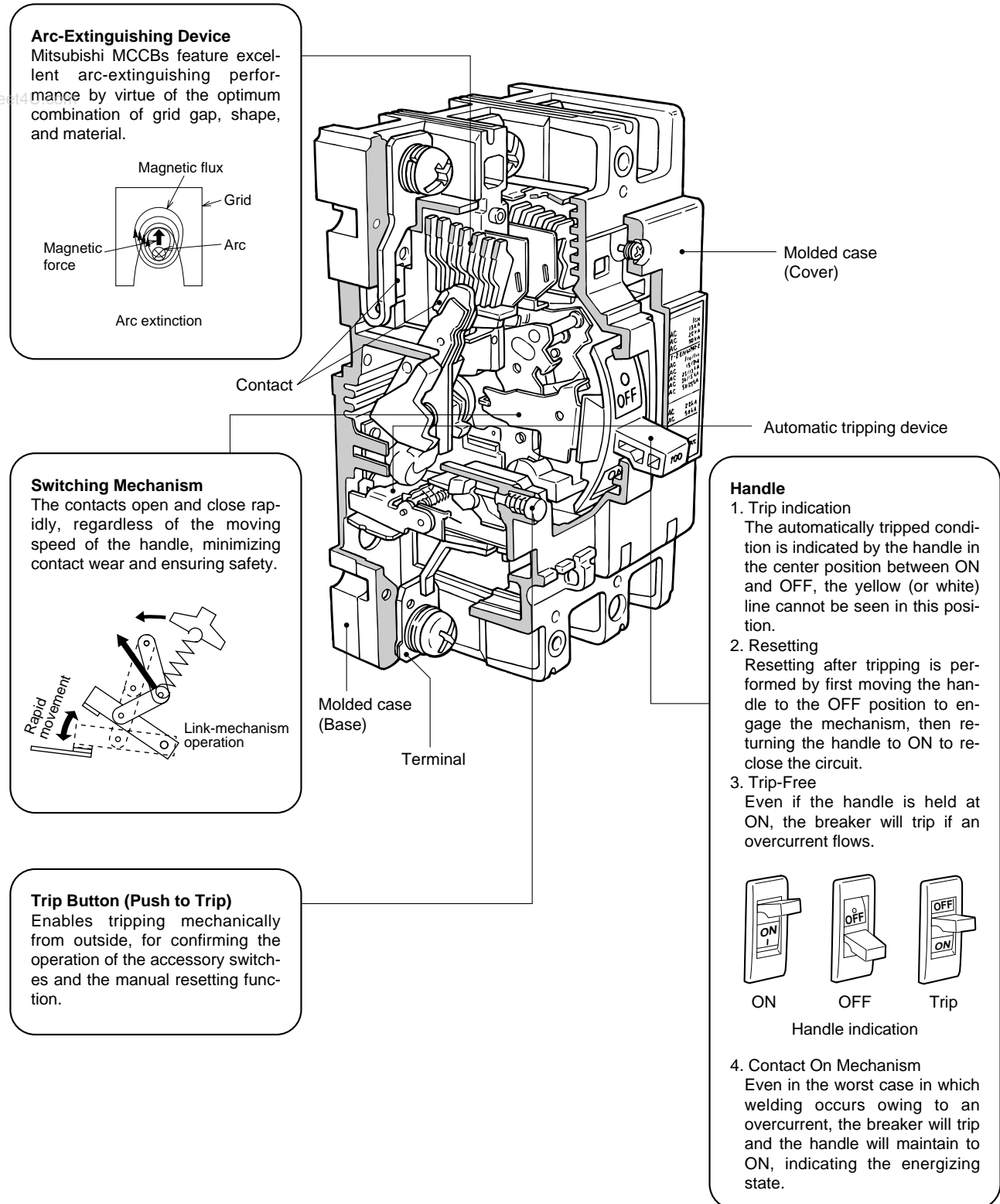
Fig. 3.1 Type NF100-SP Construction
