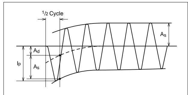
Fig. 9.3 Short-Circuit Current
