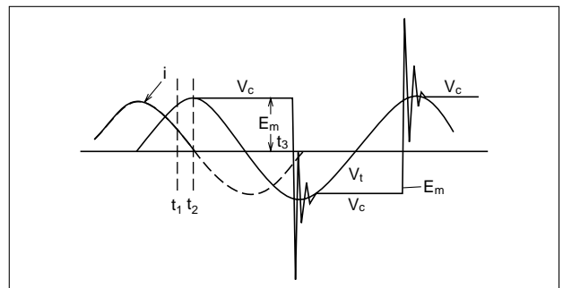
Fig. 7.9 Circuit-Opening Conditions
