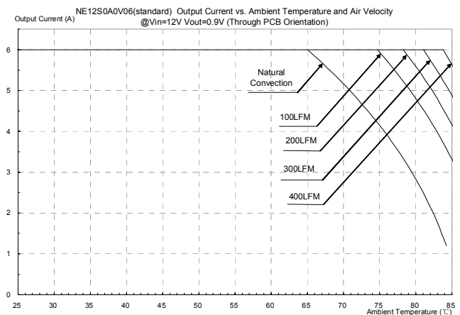
Figure 27: Output current vs. ambient temperature and air velocity @Vin=12V, Vout=0.9V (Through PCB Orientation)
