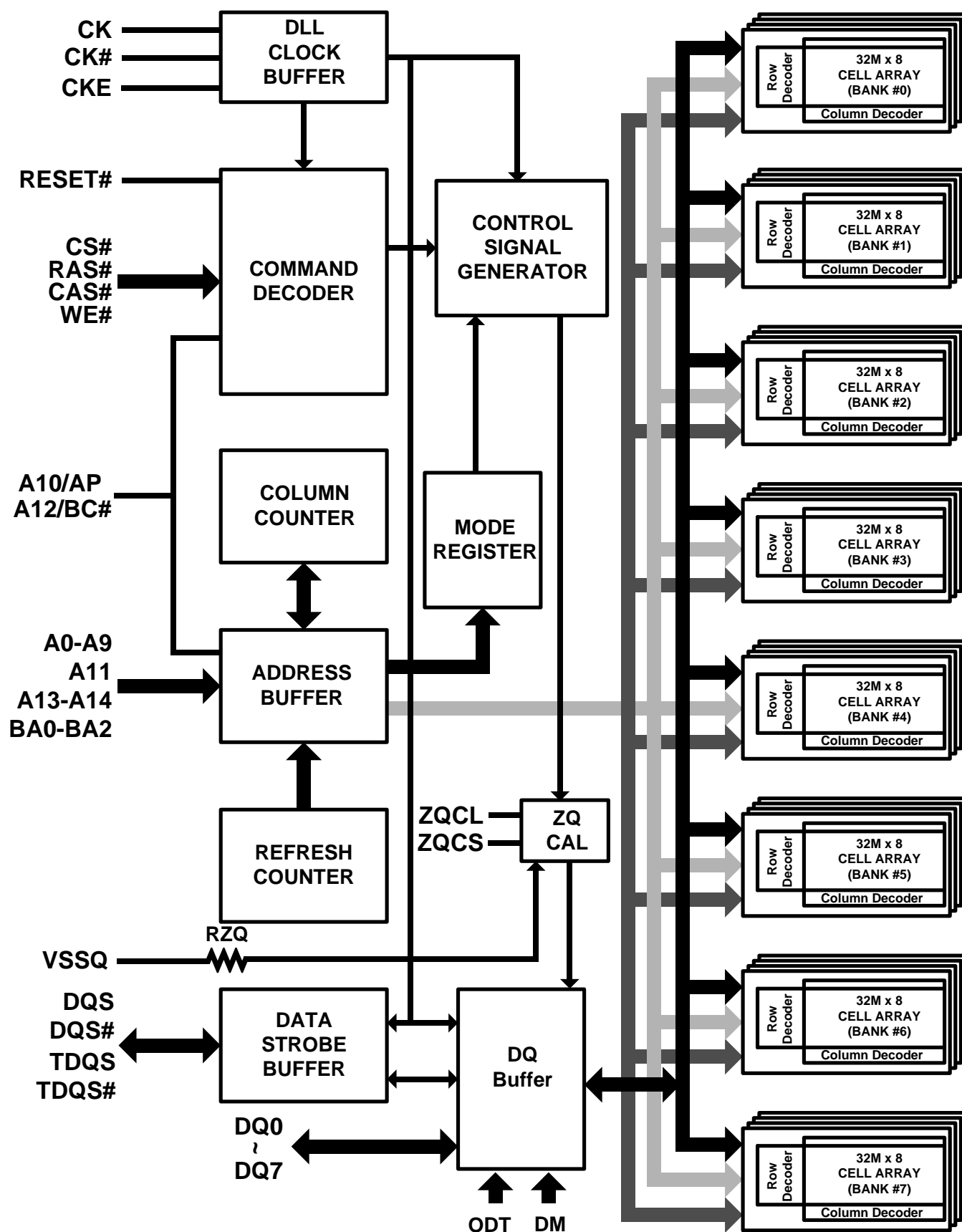
Figure 2. Block Diagram
