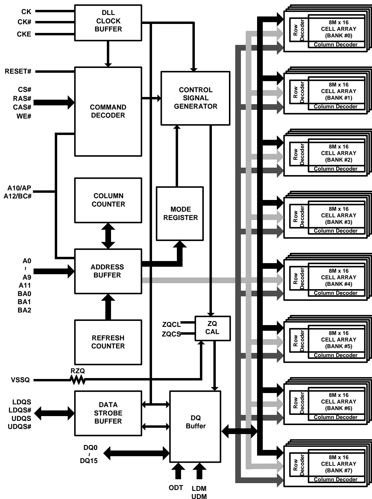
Figure 2. Block Diagram
