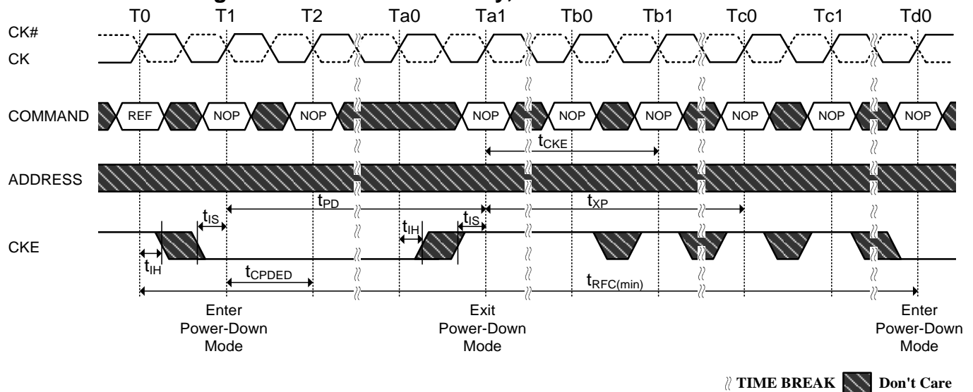
Figure 81. Power-Down Entry, Exit Clarifications-Case 3
