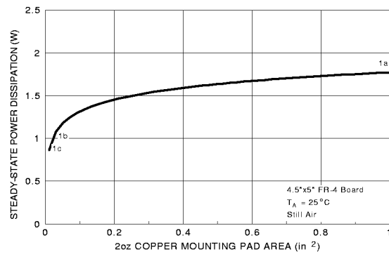
Figure 14. SOT-8 Maximum Steady-State Power Dissipation versus Copper Mounting Pad Area.
