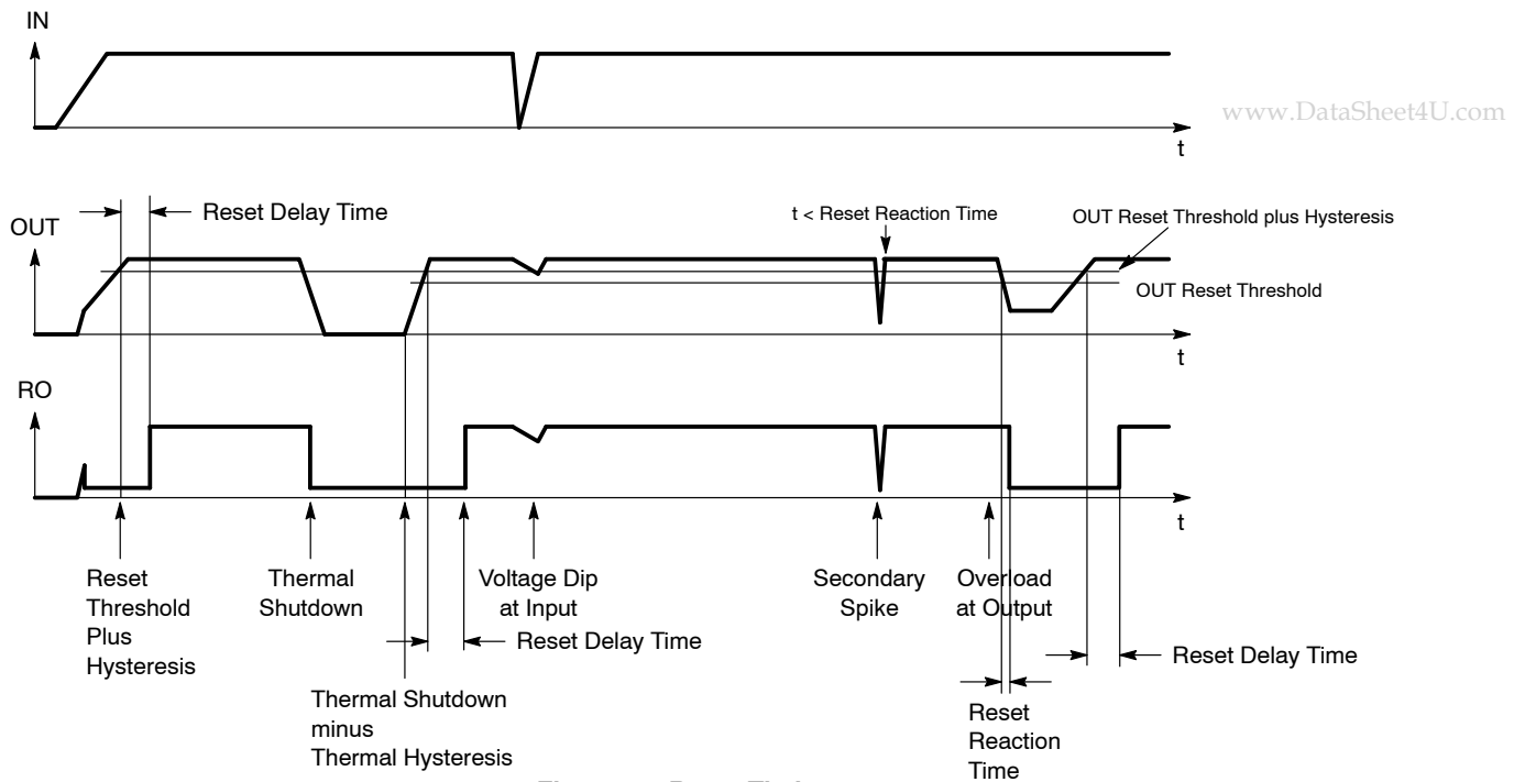
Figure 25. Reset Timing
