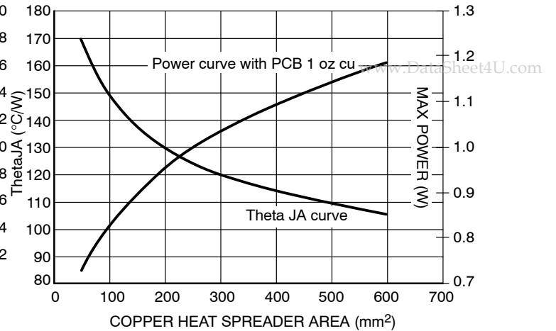
Figure 28. R_{\theta JA} vs. PCB Copper Area (SOIC-8 Fused)
