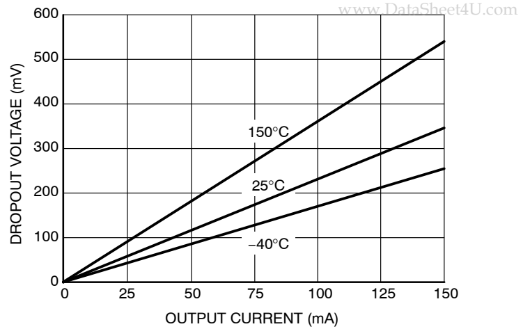
Figure 10. Dropout Voltage vs. Output Current
