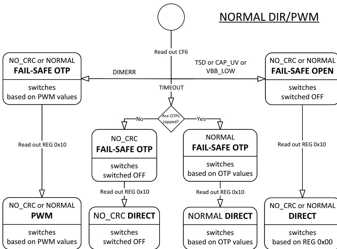
Figure 19. FAIL-SAFE Modes
