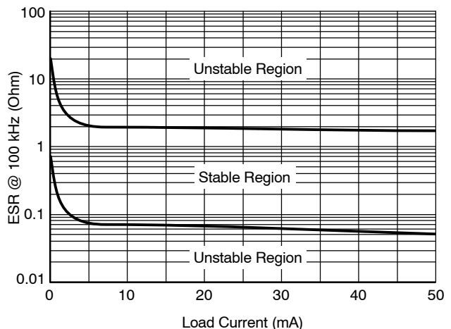
Figure 35. ESR Curves for 6.8\text{ }\mu\text{F} \leq C_L \leq 100\text{ }\mu\text{F} and Frequency of 100 kHz
