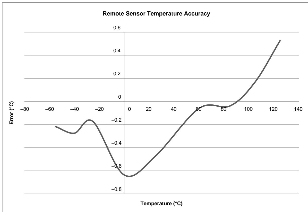
Figure 15. Remote Temperature Error vs Temperature
