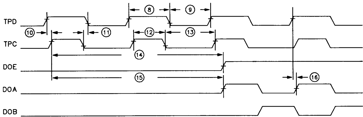
Figure 10 Receive Timing
