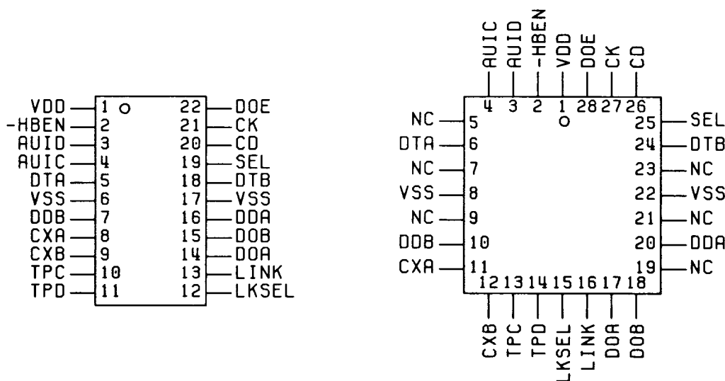
Figure 1 Pinout Diagrams
