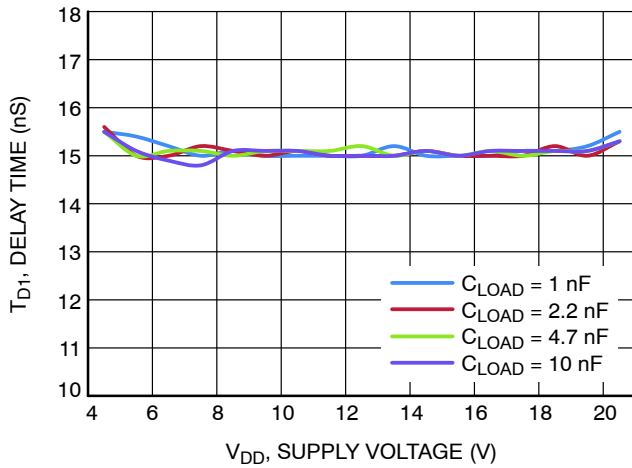
Figure 9. Propagation Delay T_{D1} vs. Supply Voltage
