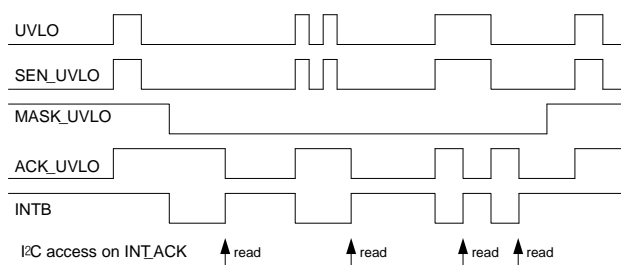
Figure 42. Interrupt Operation Example
