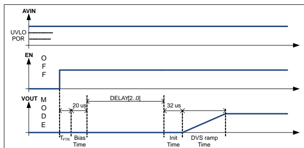
Figure 35. Normal Power Up Sequence
