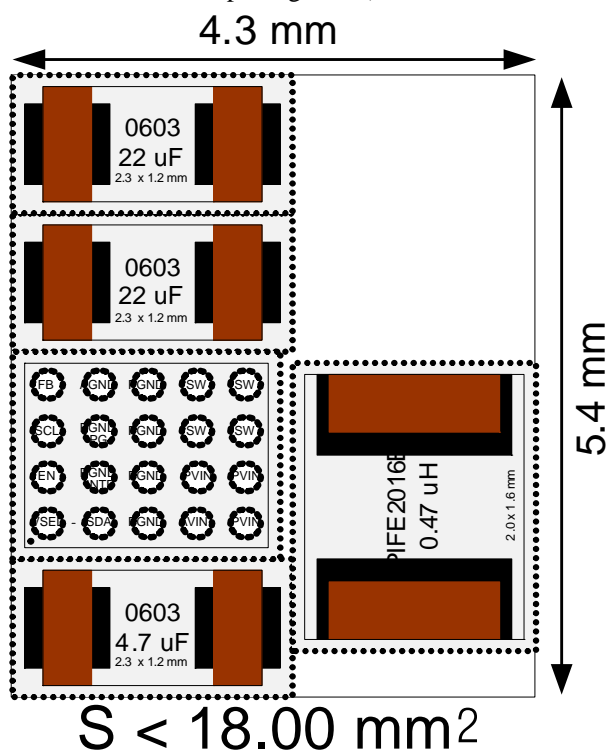
Figure 48. Layout Recommendation
