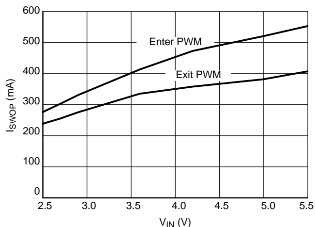
Figure 23. Switchover Point V_{OUT} = 1.39375\text{ V}
