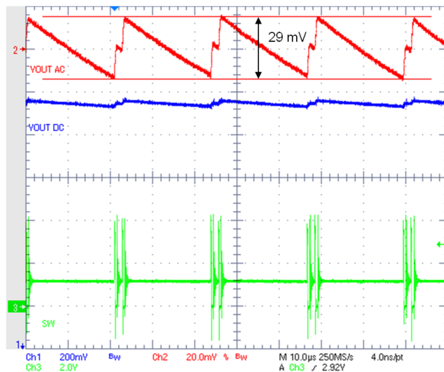
Figure 25. PFM Ripple
