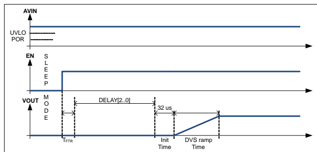
Figure 36. Quick Power Up Sequence
