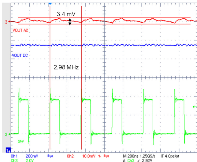
Figure 24. PWM Ripple
