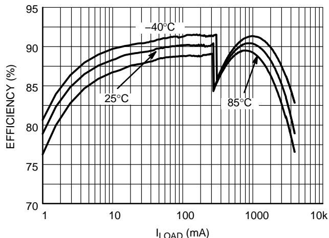
Figure 9. Efficiency vs I_{LOAD} and Temperature V_{OUT} = 0.60\text{ V} , SPM6530 Inductor
