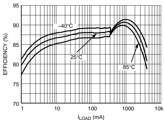
Figure 7. Efficiency vs I_{LOAD} and Temperature V_{OUT} = 1.15\text{ V} , SPM6530 Inductor
