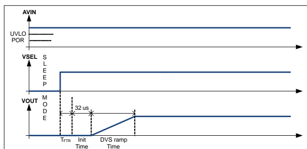
Figure 37. Fast Power Up Sequence
