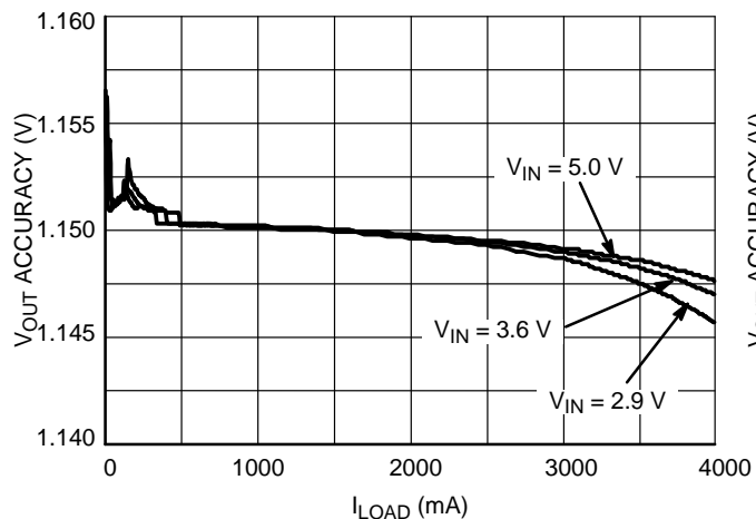
Figure 12. V_{OUT} Accuracy vs I_{LOAD} and V_{IN} V_{OUT} = 1.15\text{ V}
