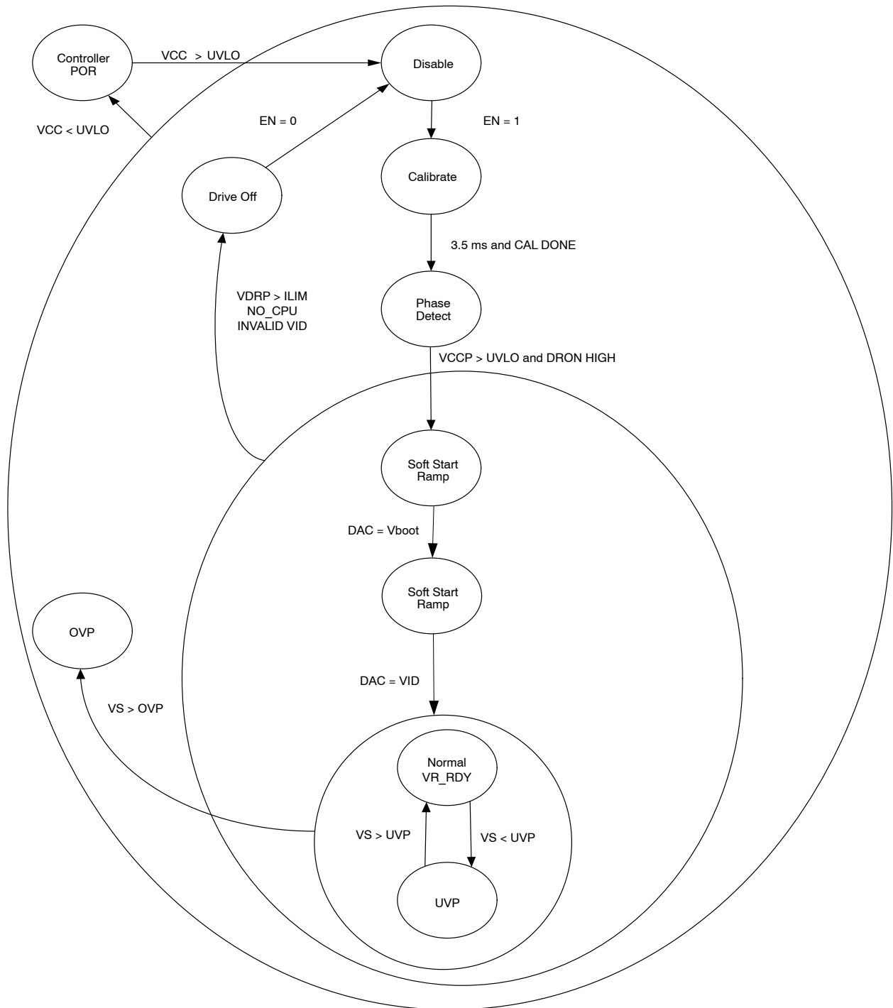
Figure 6. State Diagram
