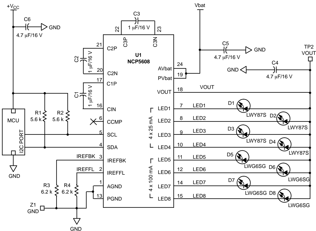
Figure 14. Typical Application
