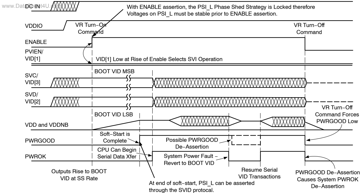
Figure 10. Power-Up Sequence in Serial Mode Operation
