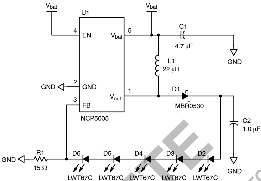
Figure 1. Typical Application
