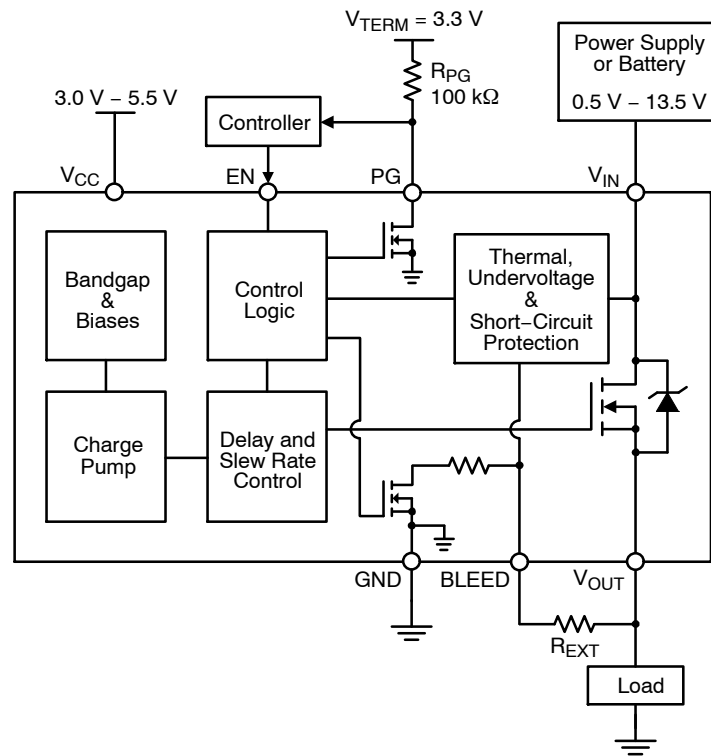
Figure 3. NCP45522 Typical Application Diagram – Load Switch
