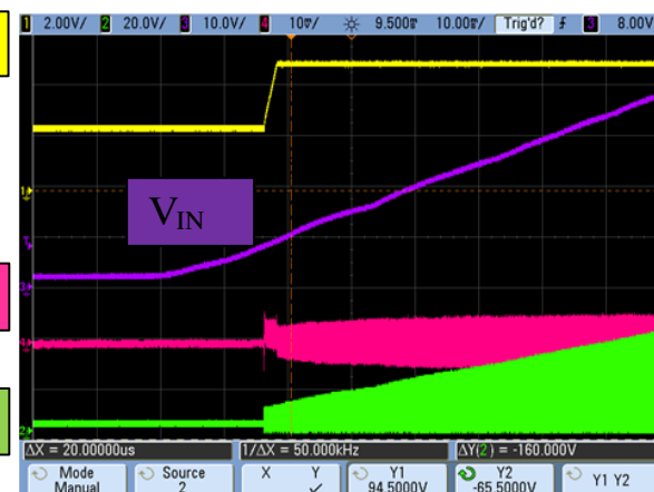
Figure 36. Start-Up with Pre-Biased Output
