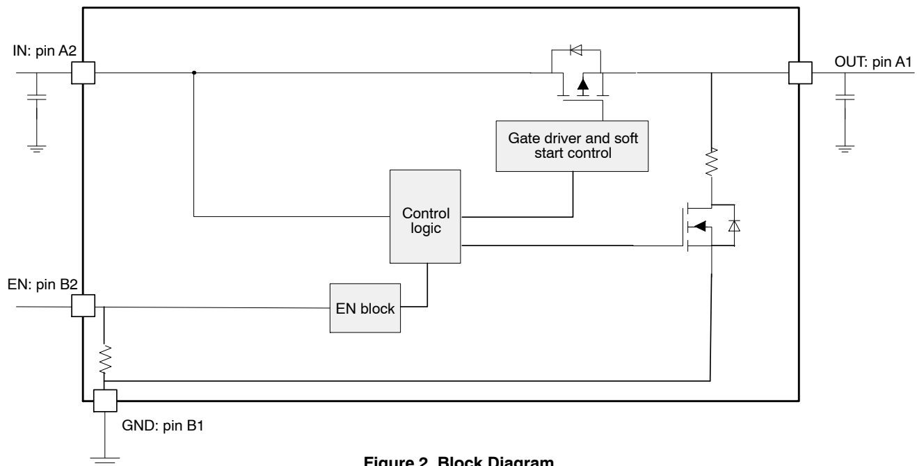
Figure 2. Block Diagram
