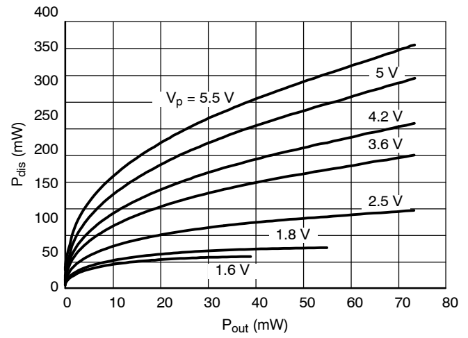
Figure 11. Power Dissipation vs P_{out} Left and Right in Phase
