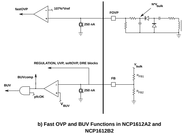
Figure 70. Bulk Under-voltage Detection
