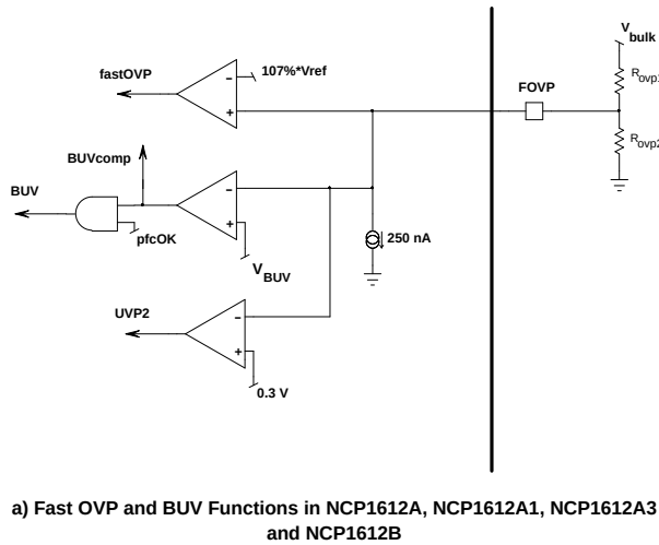
Figure 70. Bulk Under-voltage Detection
