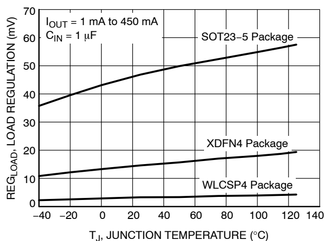
Figure 14. Load Regulation vs. Temperature
