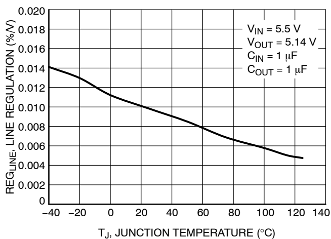
Figure 10. Line Regulation vs. Temperature – V_{OUT} = 5.14\text{ V}
