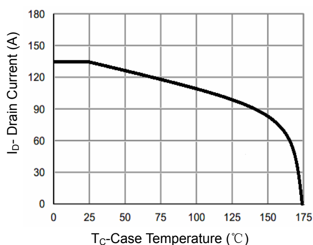
Figure 10 Current De-rating
