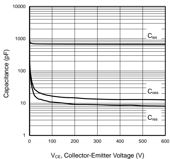
Figure 5 Capacitance Characteristics
