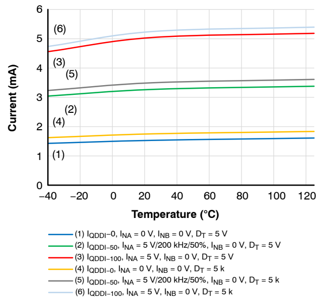
Figure 17. I_{QDDI} Supply Current, V_{DDI} = 5\text{ V}
