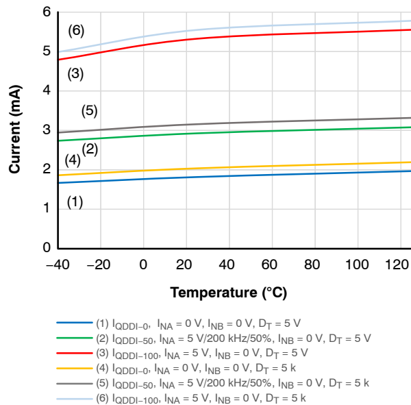
Figure 18. I_{QDDI} Supply Current, V_{DDI} = 20\text{ V}
