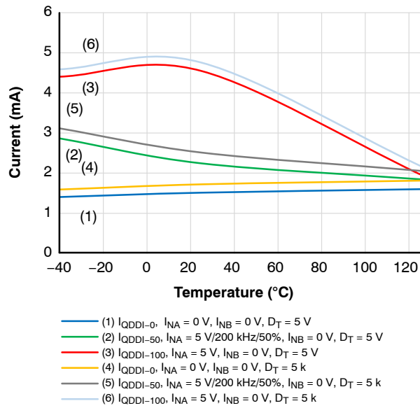
Figure 16. I_{QDDI} Supply Current, V_{DDI} = 3.3\text{ V}
