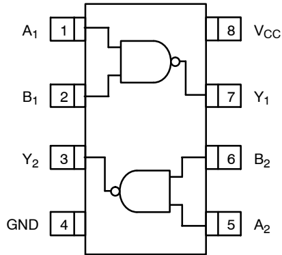
Figure 2. Connection Diagram (Top View)
