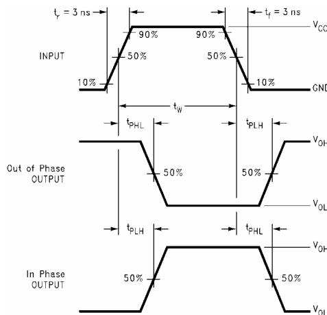
FIGURE 3. AC Waveforms
