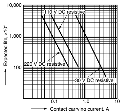
1.-(1) Life curve (2 Form C, 4 Form C)
