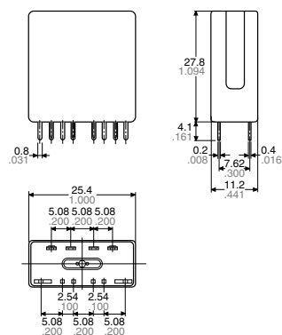
External dimensions
