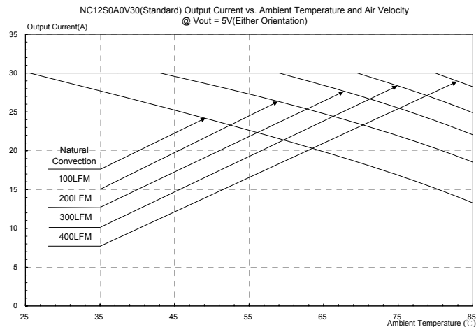
Figure 37: Output current vs. ambient temperature and air velocity @ Vout=5V(Either Orientation)
