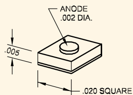
CH1 Chip (inches)
