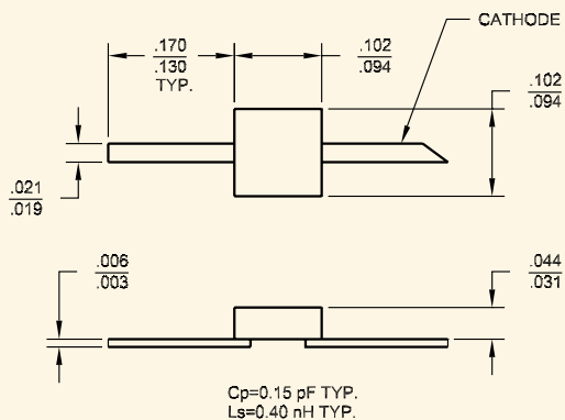
BL Package (inches)
