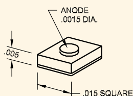
CH2 Chip (inches)
