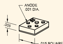
CH3 Chip (inches)
