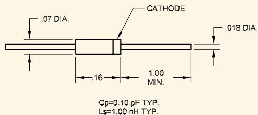
DO-35 Package (inches)
