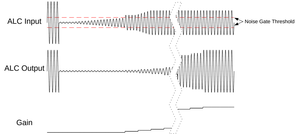
Figure 6: ALC with noise gate
