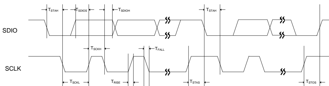
Figure 30: Two-wire Control Mode Timing
