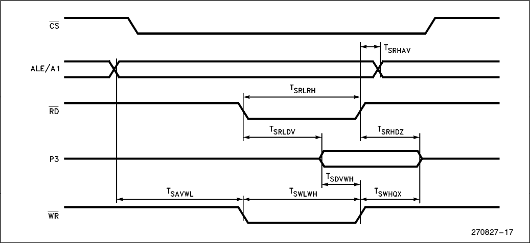
SLAVE PORT WAVEFORM—(SLPL = 0)
