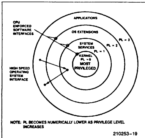
Figure 19. Four-Level Privilege
