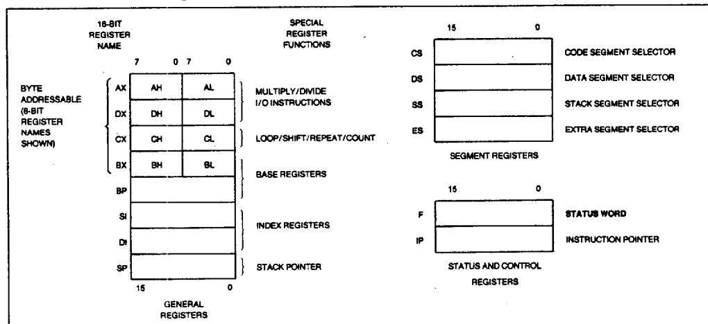
Figure 3. Register Set
