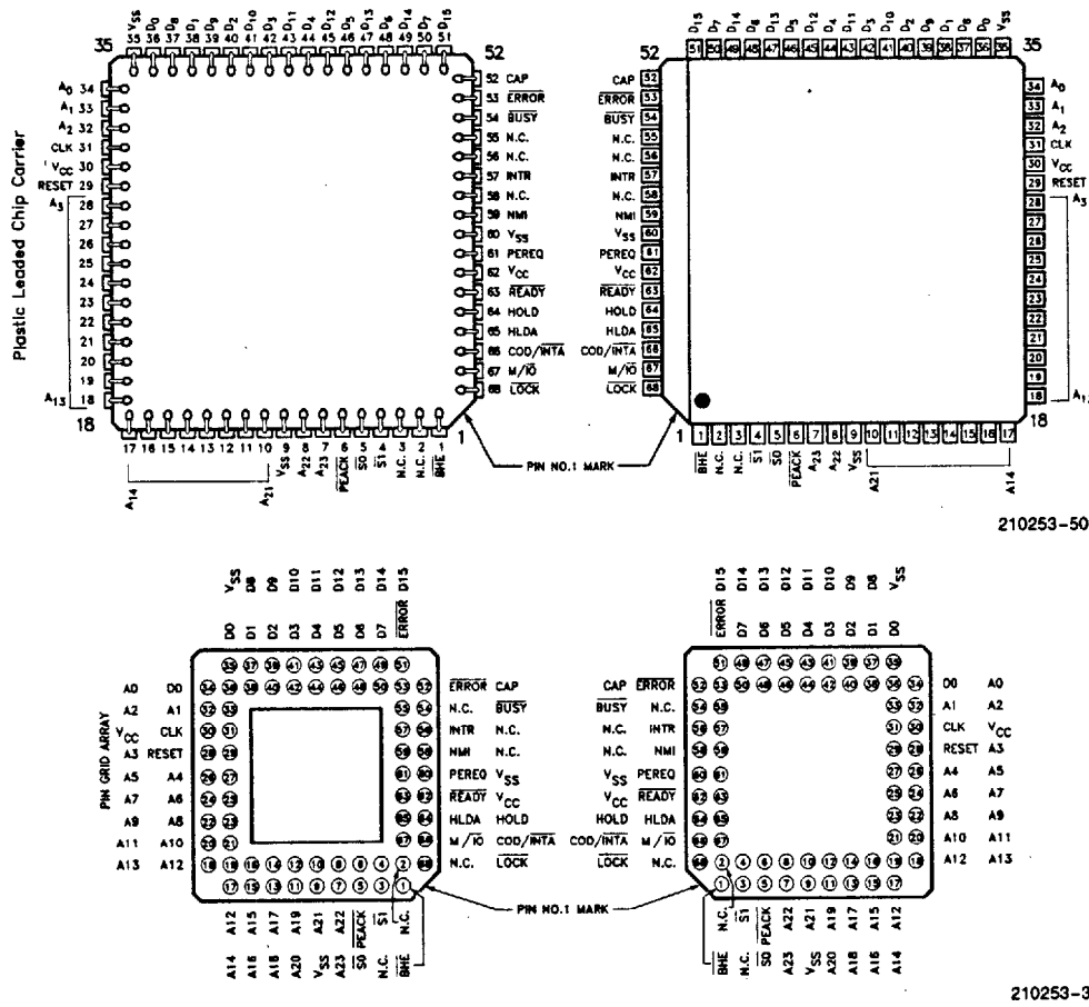
Figure 2. 80286 Pin Configuration
