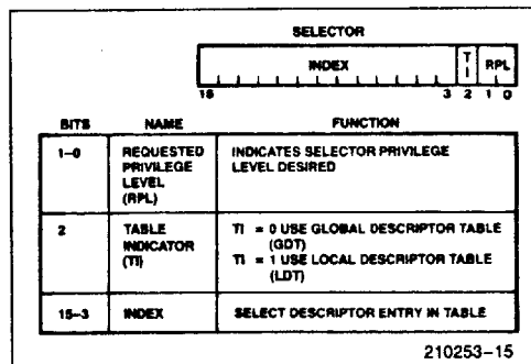
Figure 15. Selector Fields
