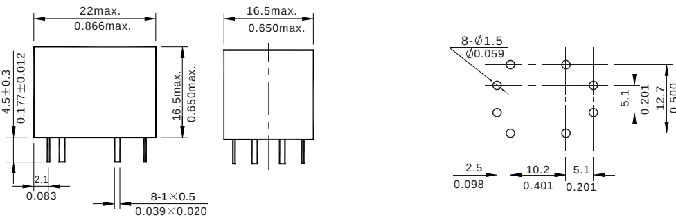
Mounting (Bottom view)
