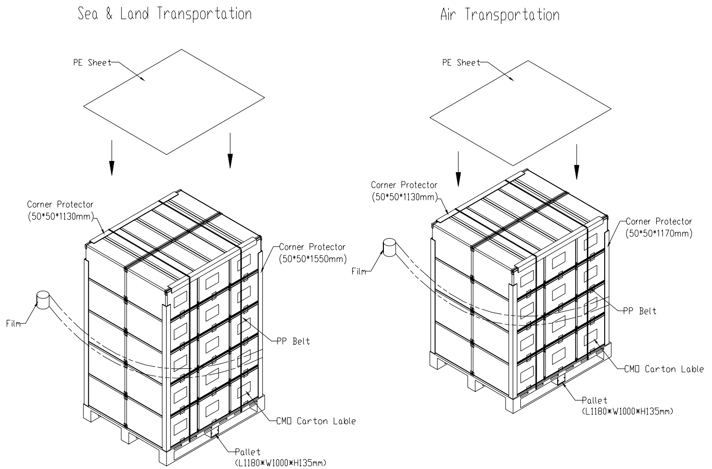
Figure. 10-2 Packing method
