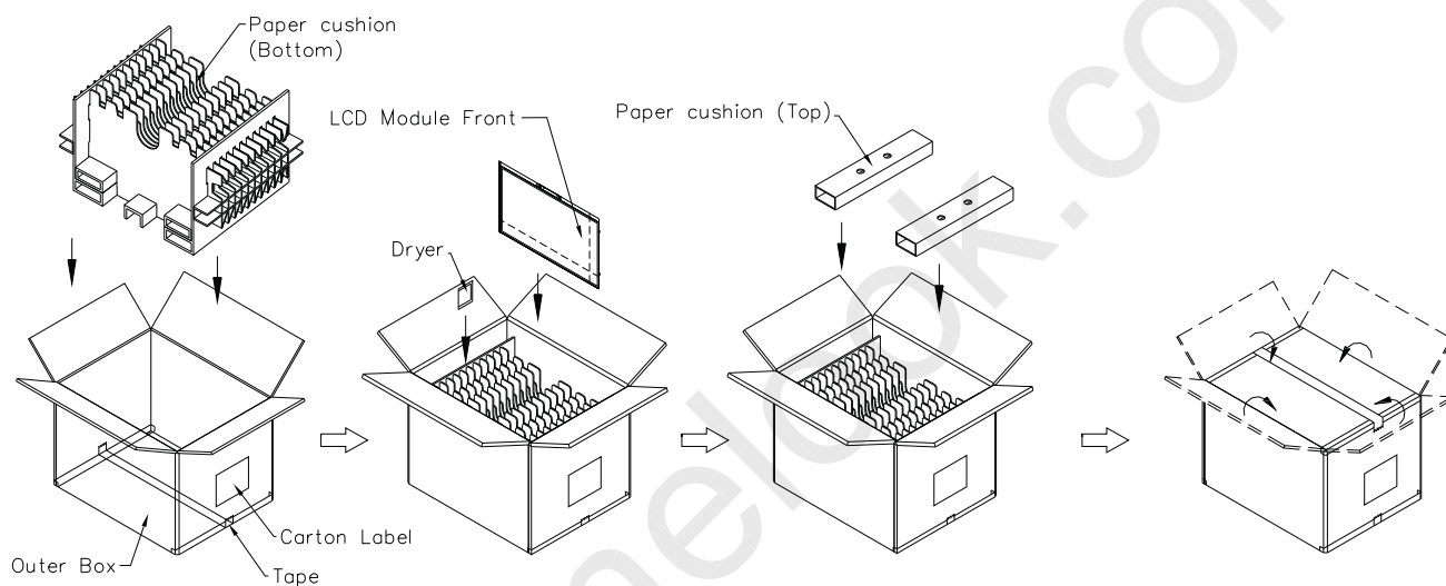
Figure. 9-1 Packing method
