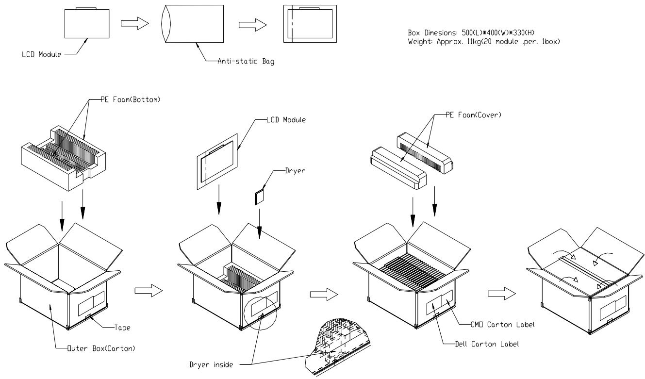
Figure. 9-1 Packing method
