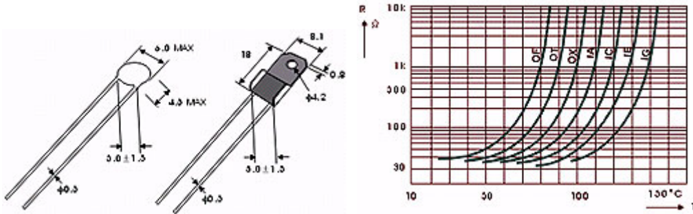
Fig.1 Component outline
